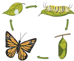
life cycle
