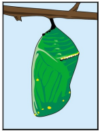
Chrysalis/cocoon
