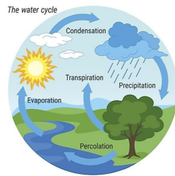
the water cycle
